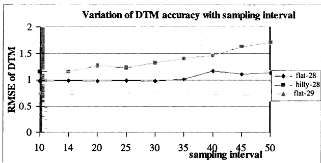
Figure 4. Effect of sampling interval on DEM accuracy.
