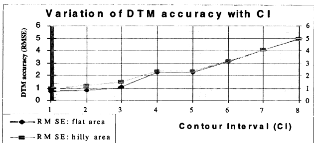
Figure 5. Variation of DEM accuracy with contour intervals.
