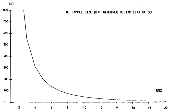
FIG. 1. Sample size (number of check points) with required accuracy.
