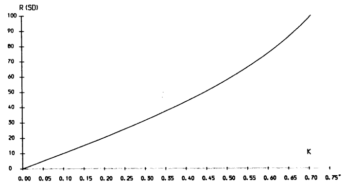
Fig. 5. The reliability of the estimated SD of the DTM with the accuracy of the check points (in terms of the ratio of the SD of the check points to that of the DTM).
