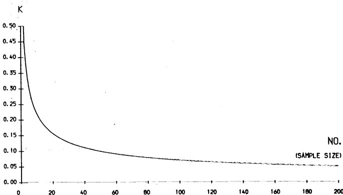
Fig. 4. Required accuracy of check points (in terms of the ratio of the SD of check points to that of the DTM) with sample size.
