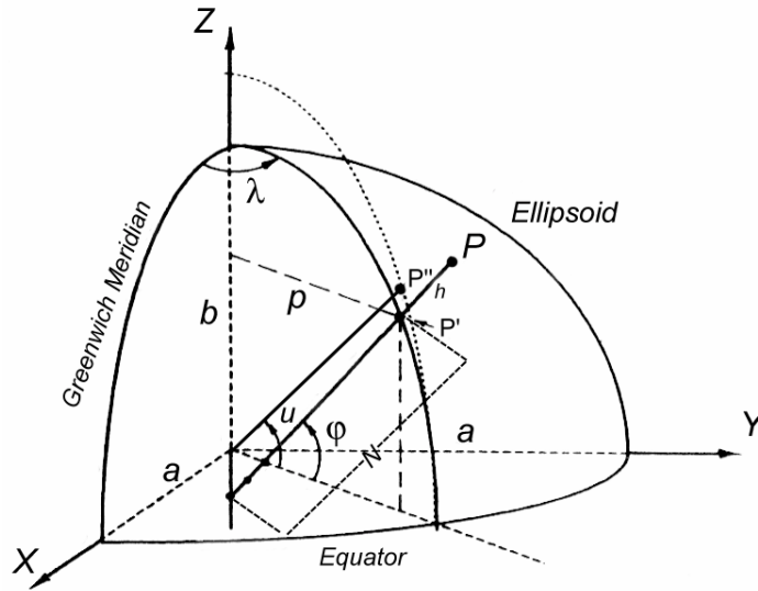
Figure 1. Geodetic and Cartesian Coordinates.
